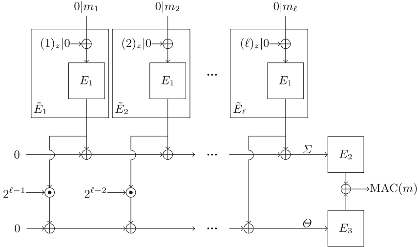
Fig. 5. Diagram for LightMAC+ with (n - z) -bit blocks of a \ell -block message where (v)_z is the value v written over z bits.
