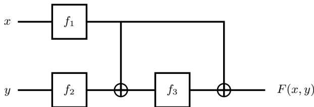
Fig. 1. The Shrimpton-Stam compression function. All wires carry n -bit values.
